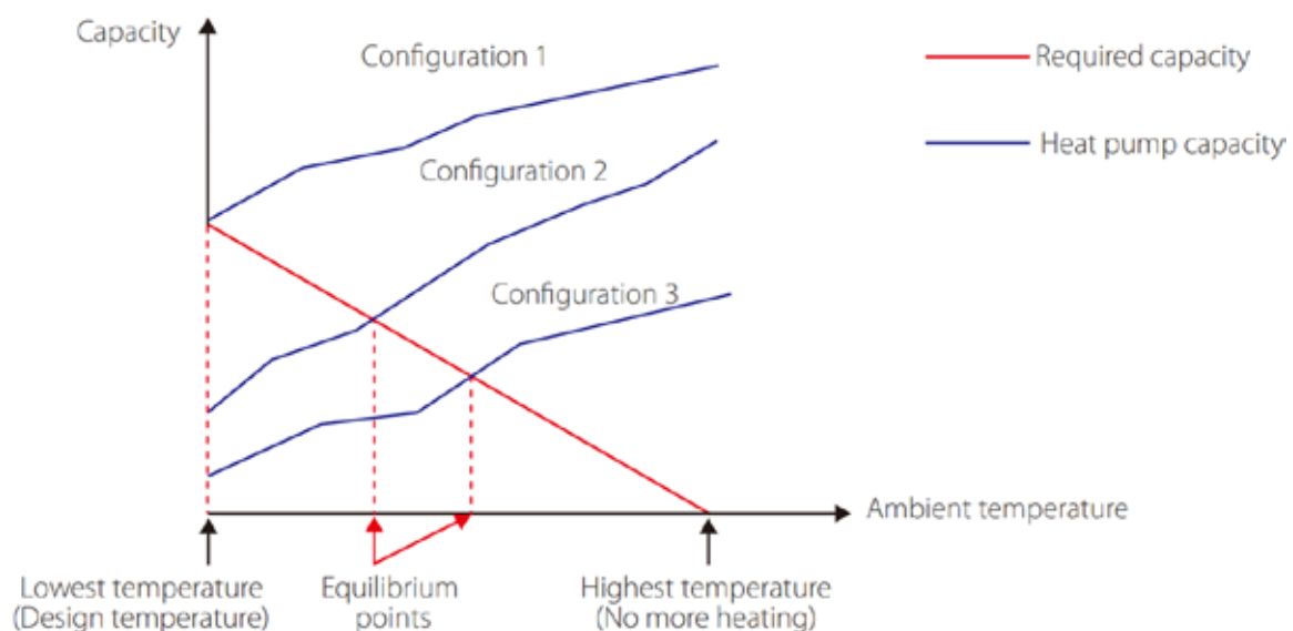
Figure 1-1.2: System configurations
